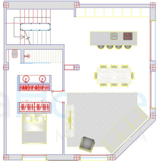
Upper Floor
